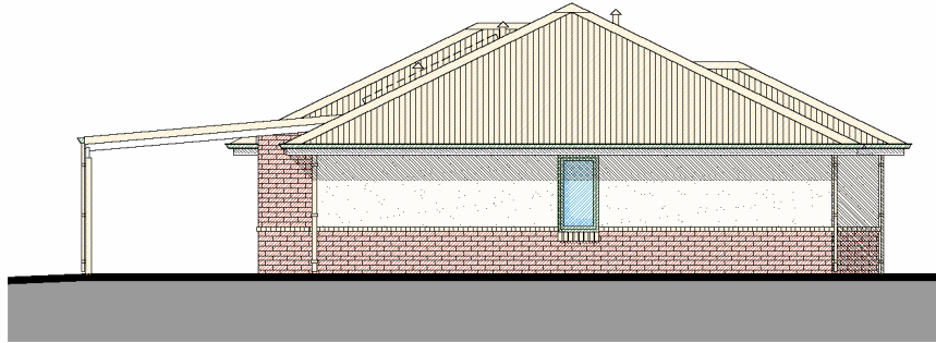
REAR ELEVATION
