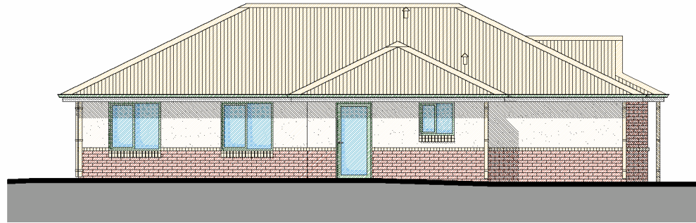
SIDE ELEVATION
