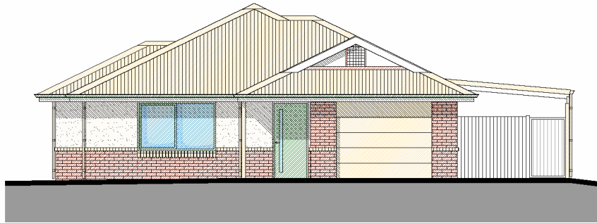
FRONT ELEVATION
